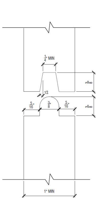
FIGURE 1A—TONGUE AND GROOVE FOAM BOARD
